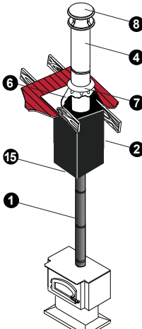
Cathedral Ceiling Roof Support
